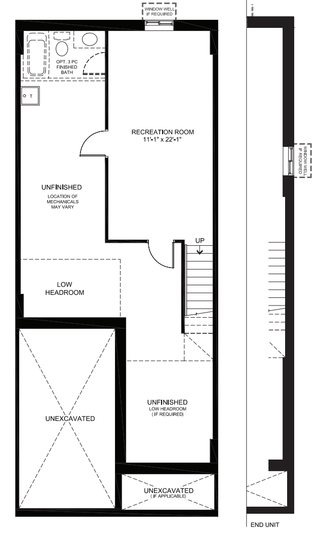
FINISHED BASEMENT
